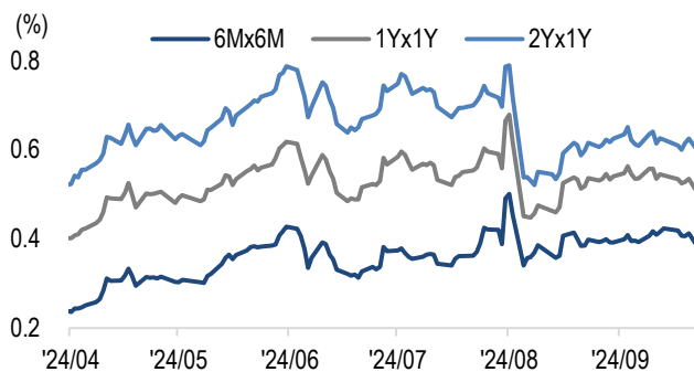
Figure 99: We would consider paying 1Yx1Y when it dips a few basis points below 50bp
