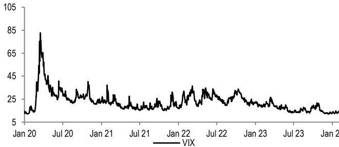
Figure 42: VIX
