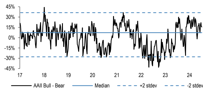
Figure 37: AAI Bull-Bear
