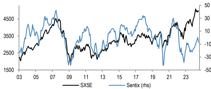
Figure 41: Sentix Sentiment Index vs SX5E
