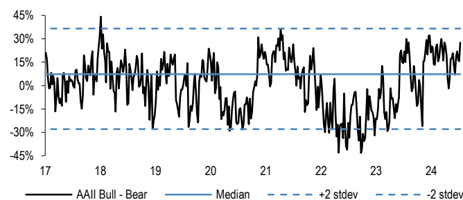
Figure 39: AAI Bull-Bear
