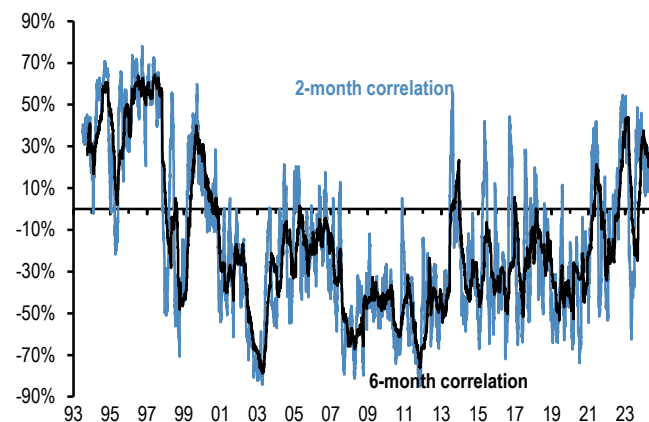
Figure 9: Bond/Equity correlation
