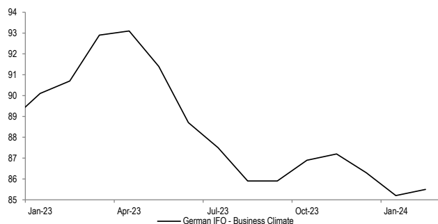
Figure 23: German IFO
