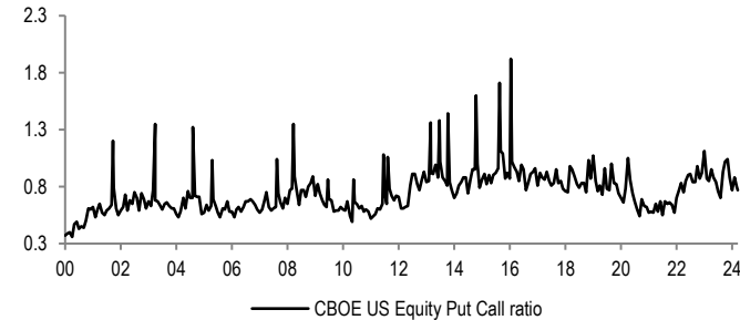
Figure 38: Put-call ratio
