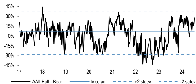
Figure 39: AAI Bull-Bear
