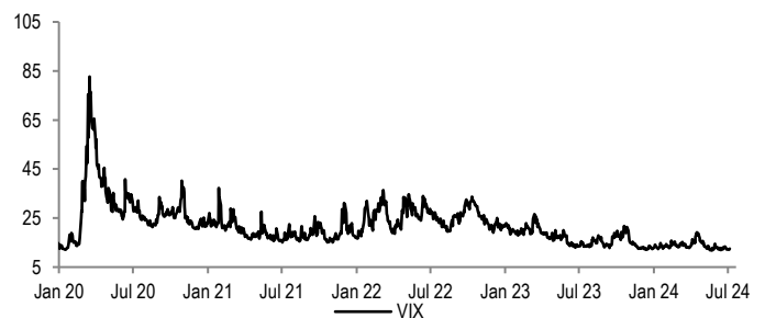
Figure 42: VIX
