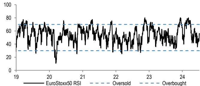
Figure 36: EuroStoxx50 RSI
