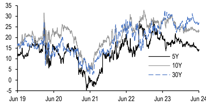
Figure 19: ...and IOTAs have narrowed over the past year, primarily in the 5- and 10-year sectors, despite ongoing QT IOTA (from Z-spread to SOFR differential) for 5-, 10-, and 30-year TIPS; bp
