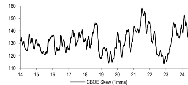
Figure 42: Equity Skew
