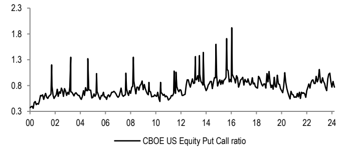
Figure 38: Put-call ratio
