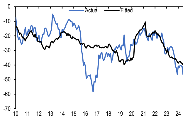
Figure 18: Actual vs. fitted 10y US swap spread
