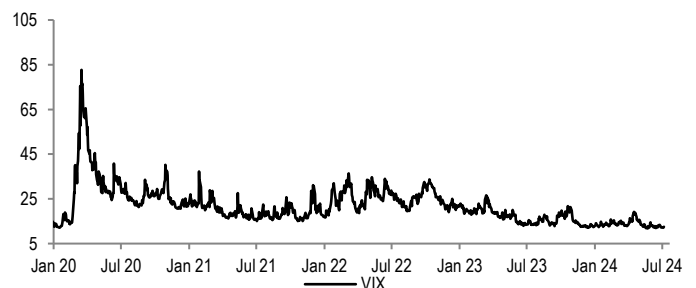
Figure 42: VIX
