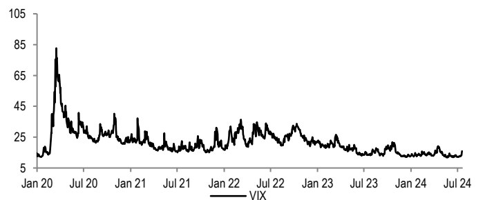
Figure 53: VIX
