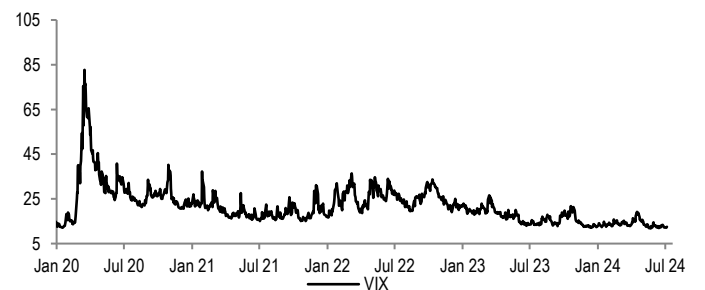
Figure 42: VIX
