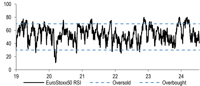
Figure 47: EuroStoxx50 RSI
