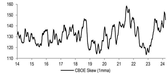
Figure 40: Equity Skew
