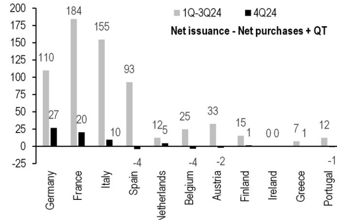
Figure 20: Pressure on primary markets to ease materially in 4Q24 despite ongoing APP & partial PEPP QT
