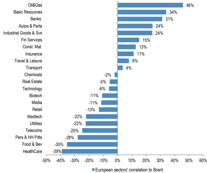
Figure 18: European sectors' correlation to Brent
