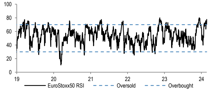
Figure 33: EuroStoxx50 RSI
