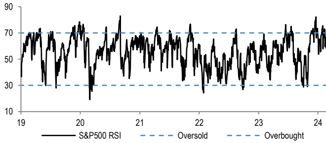
Figure 32: S&P500 RSI
