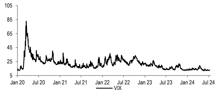
Figure 44: VIX
