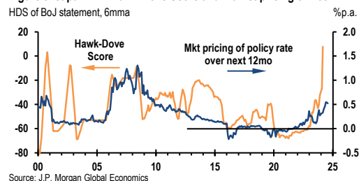
Figure 3: Japan NLP Hawk-Dove Score and market pricing of BoJ HDS of BoJ statement, 6mma
