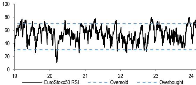
Figure 33: EuroStoxx50 RSI
