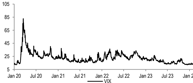
Figure 39: VIX
