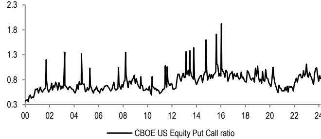
Figure 35: Put-call ratio
