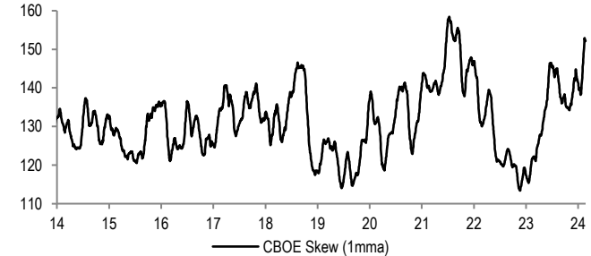
Figure 37: Equity Skew
